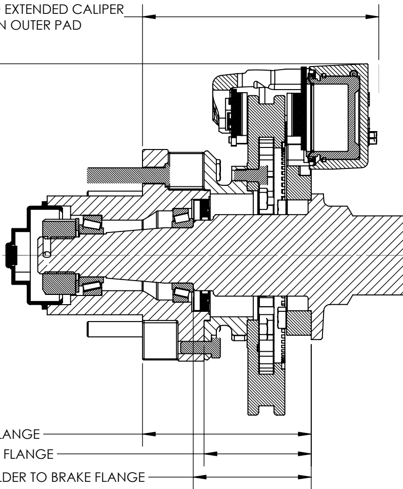
SECTION B-B
